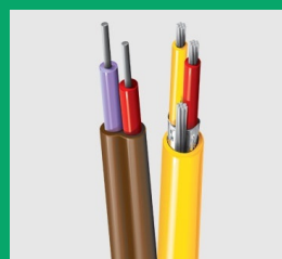
Tech Tips- Identifying Thermocouples Using Magnet Page 6
