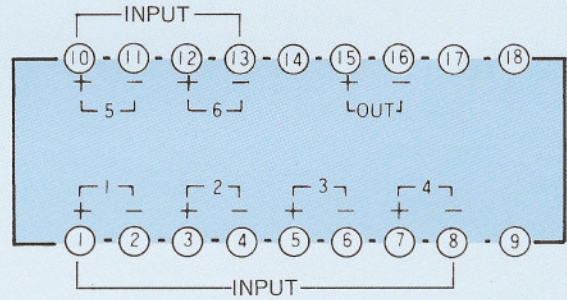
KR15A
