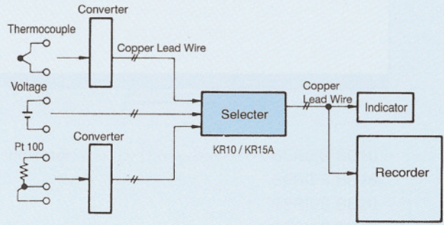
Selection of Voltage (KR10, KR15A)
