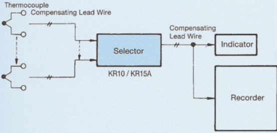
Selection of Thermocouple (KR10, KR15A)
