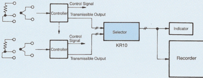
Selection of Transmissible Output (KR10, KR15A)
