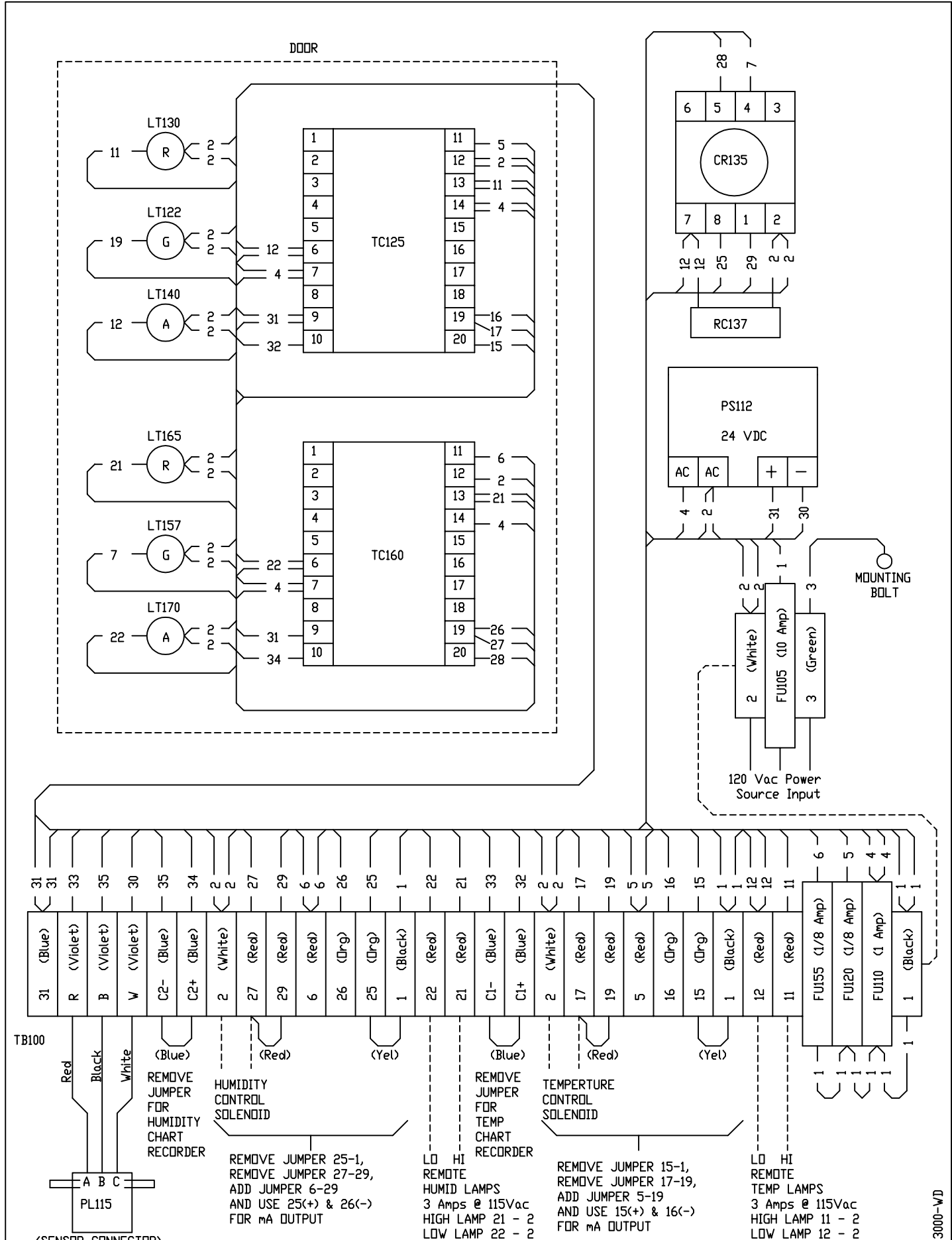
PROOFER CONTROL SYSTEM WIRING DIAGRAM, PCS-3000 W. H. COOKE & CO., INC. 10 MAR 2008 (Love 4B)
